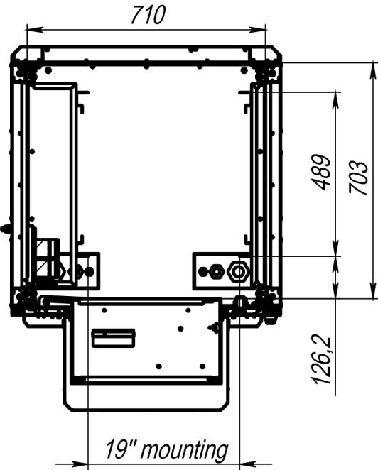
B-B Internal dimensions
