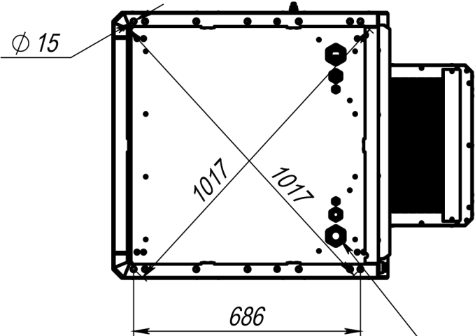
Mounting holes
