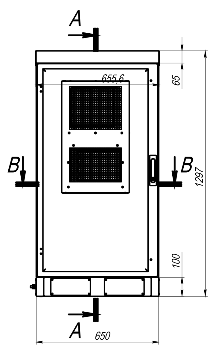
B-B Internal dimensions
