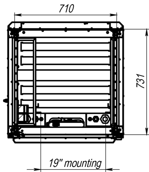
B-B Internal dimensions
