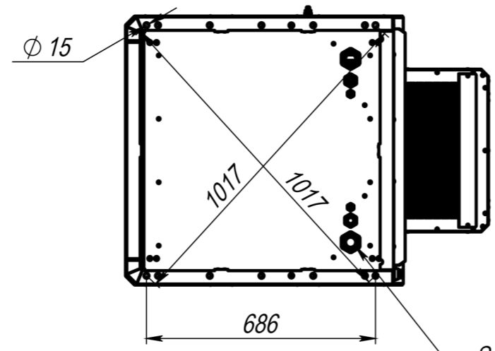
Mounting holes
