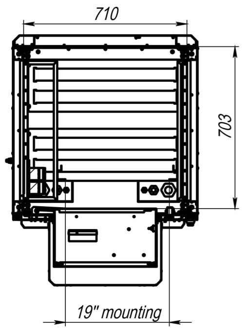
B-B Internal dimensions
