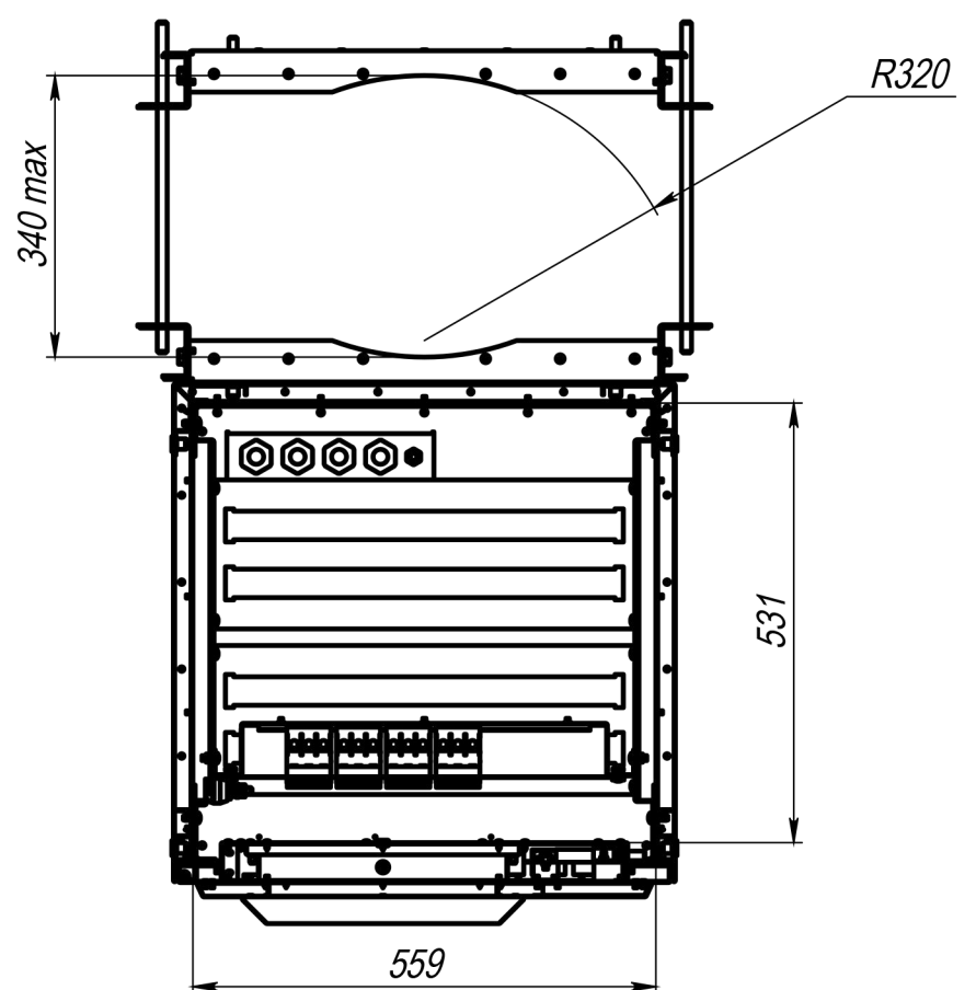
B-B Internal dimensions
