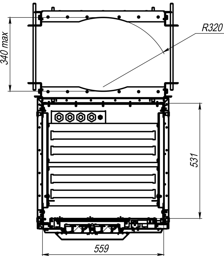
B-B Internal dimensions
