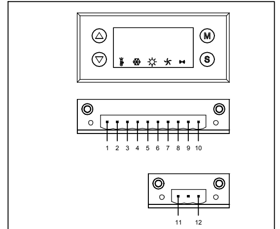
Figure 3 - Wiring interface with customer circuit
