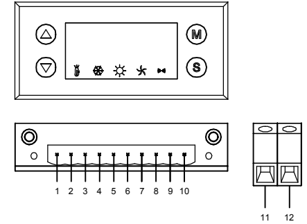
Figure 3 - Wiring interface with customer circuit
