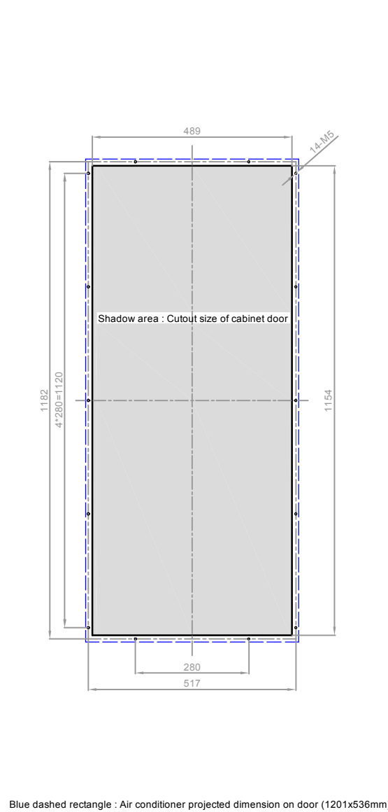
Figure 2 - Mounting interface with cabinet door
