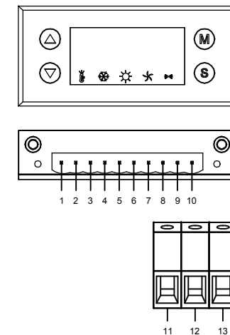
Figure 3 - Wiring interface with customer circuit
