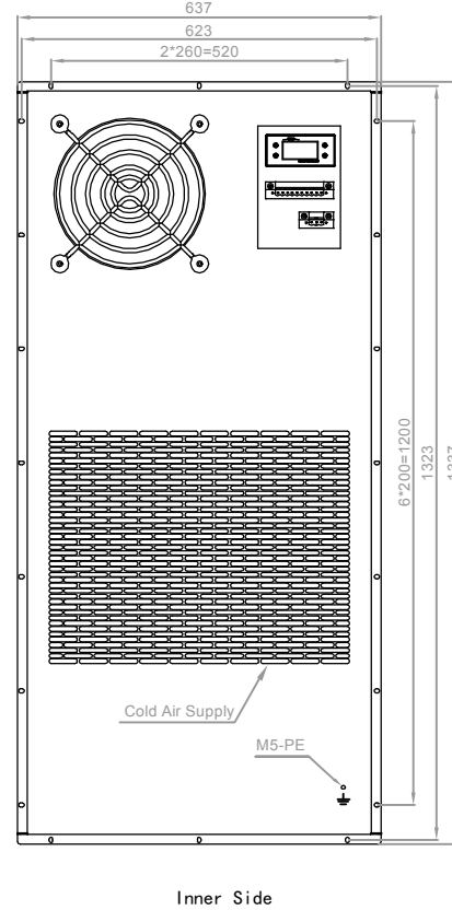
Inner Side
