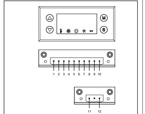
Figure 3 - Wiring interface with customer circuit
